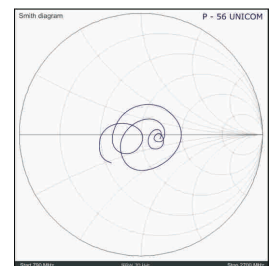
Smith diagram Smithov diagram:
